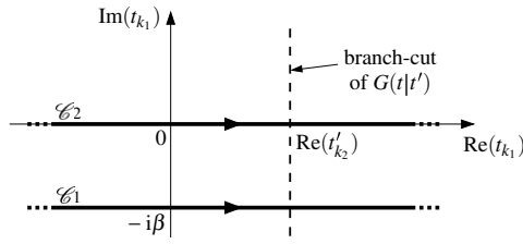
Figure 3. If an annihilation operator at time t_{k_1} and a creation operator at time t'_{k_2} are of the same state and are situated on the same branch of the contour, then the Green's function G(t|t') has a branch-cut along \text{Re}(t_{k_1}) = \text{Re}(t'_{k_2}) . In this case the Fourier integrals of G(t|t') over t_{k_1} along the paths \mathcal{C}_1 and \mathcal{C}_2 are not equal.
