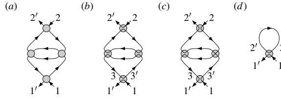
Figure 2. Examples for the application of the diagram rules. The lines are free one-particle Green’s functions, and the dots are interaction vertices. The indices represent contour index, state and frequency, e.g. 1 = (j_1, q_1, \omega_1) . The diagram (a) contributes to the two-particle vertex function. It has one pair of equivalent lines, n_{\text{eq}} = 1 , and no symmetries, S = 1 . (b) and (c) show two possible, equivalent ways to assign the lines to the indices of the vertices. In (b) the vertex at the bottom, e.g., is \bar{v}_{1'3'|13} , and n_{\text{loop}} = 2 , \zeta^P = 1 . In (c), the vertex at the bottom is \bar{v}_{1'3'|31} = \zeta \bar{v}_{1'3'|13} , and n_{\text{loop}} = 0 , \zeta^P = \zeta . Compared to (b), three of the four vertices acquire a factor \zeta ; taking into account the prefactor \zeta^{n_{\text{loop}}}\zeta^P , the possibilities (b) and (c) hence lead to the same value of the diagram. The Hartree–Fock diagram (d) ( n_{\text{eq}} = 0 , S = 1 ) contributes to the one-particle vertex, that is the self-energy. The figure shows the evaluation with vertex \bar{v}_{1'2'|12} and n_{\text{loop}} = 1 .
