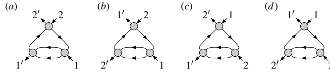
Figure 4. Examples of diagrams contributing to the two-particle vertex function \gamma_{1'2'|12} . The external indices represent the contour index, state and frequency, e.g. 1 = (j_1, q_1, \omega_1) .
