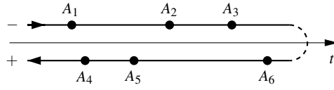
Figure 1. The time contour consisting of the - and the + branch with some example operators A_1, \dots, A_6 . The time ordering operator T_c will establish the order A_4 A_5 A_6 A_3 A_2 A_1 . The operator \tilde{T}_c used in definition (41) of the tilde Green's function will establish the order A_6 A_5 A_4 A_1 A_2 A_3 .
